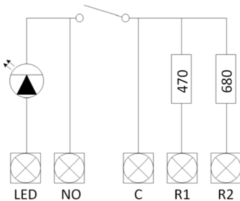
Terminal Layout
